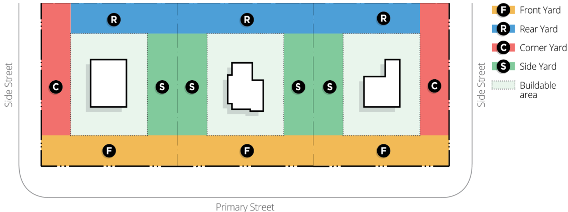
Figure 4-1: Yard Setback Locations
